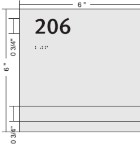
Room Sign w/Slot - Type 3B
