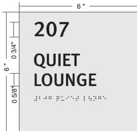
Room Sign - Type 3C
