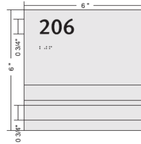
Room Sign w/2 Slots - Type 3A-2
